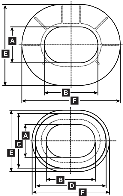
UMC-1218E - Mooring Eye 12" x 18"
